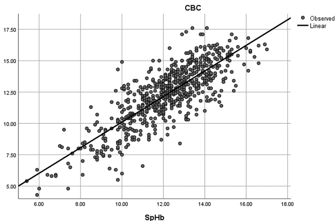
Fig. 2. Linear regression.
